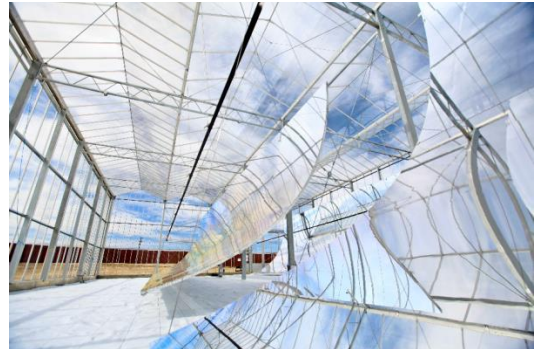
GlassPoint – Solar steam generators for the oil & gas industry
